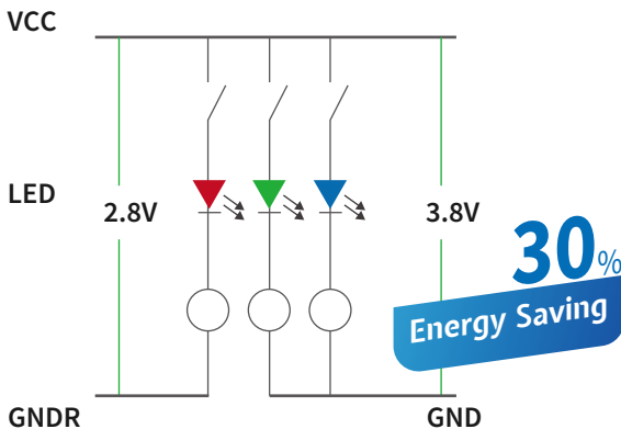
Energy-Saving Voltage Divider Design
